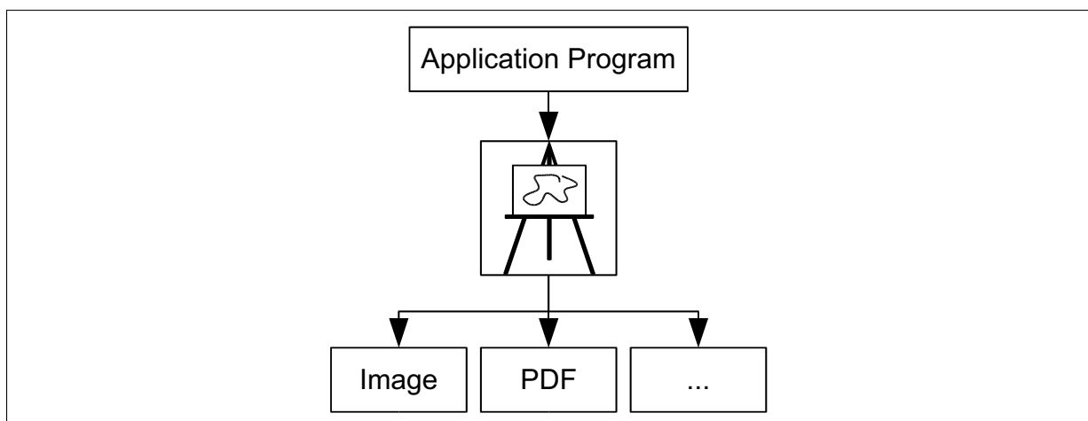
Figure 4.3: Canvas Abstraction
