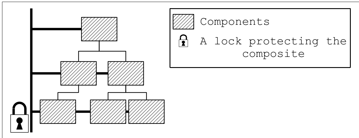
Figure 6.5: Hierarchy Lock
